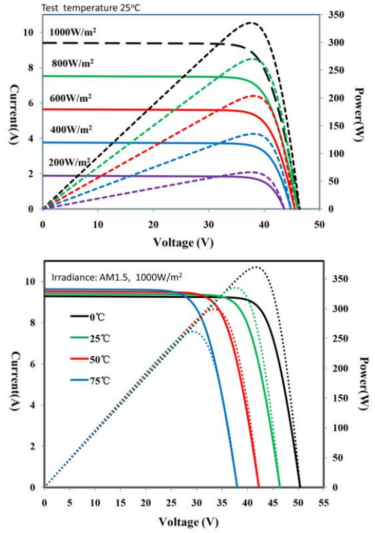
I-V Curve
