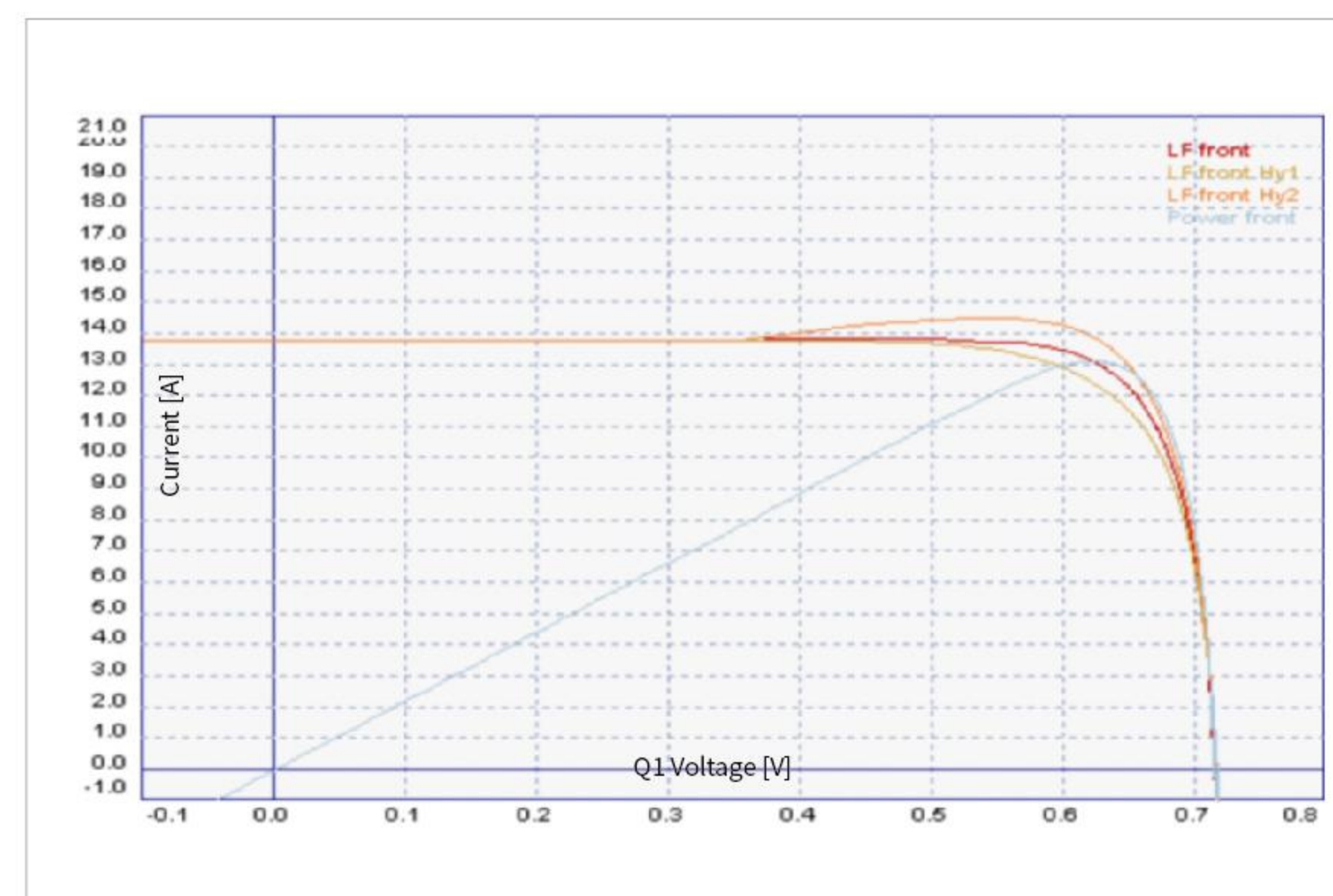
Front IV Curve
